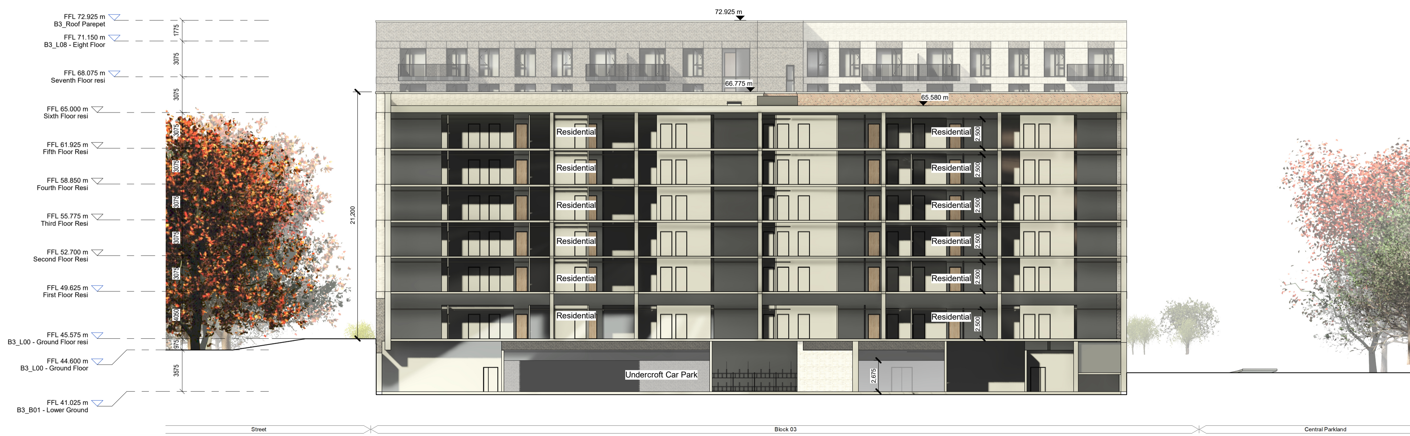
Block 03, Section B - B 1 : 200
